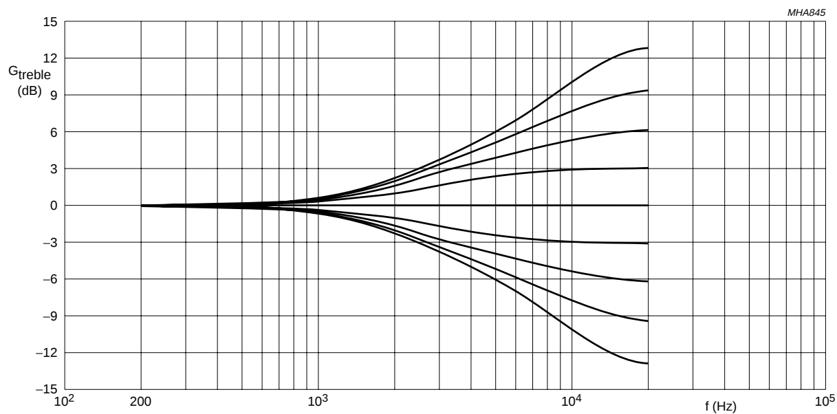
Fig.8 Treble control.
